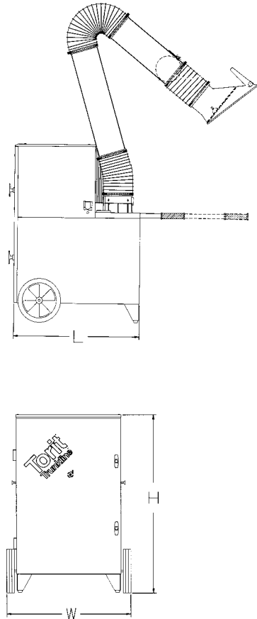
Porta-Trunk Collector
